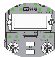
M12 D-Code, ETHERCAT Net_In/Out 接线示意
