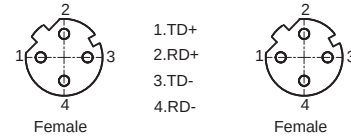
M12 D-coded Female, PROFINET Link 1/2 接线示意
