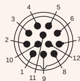
M23 12-Pin
