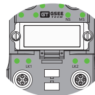
M12 D-Code, ETHERNET/IP Link 1/2 接线示意
