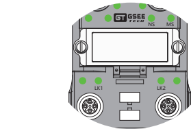
M12 D-Code, Modbus TCP Link 1/2 接线示意
