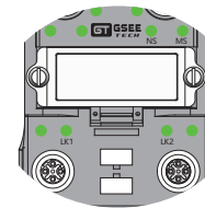
M12 D-Code, PROFINET Link 1/2 接线示意
