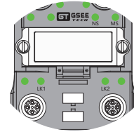
M12 D-Code, ETHERNET/IP Link 1/2 接线示意
