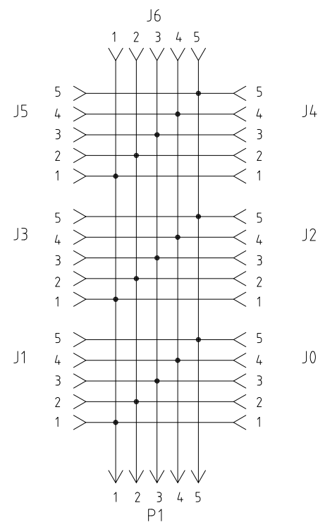
WIRING DIAGRAM
